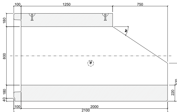
PATKOVÁ TROUBA TYP-ZP 80/200/125 SH
