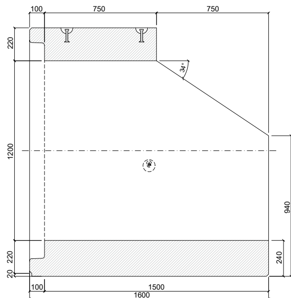
PATKOVÁ TROUBA TZP-ZP 120/150/75 SH
