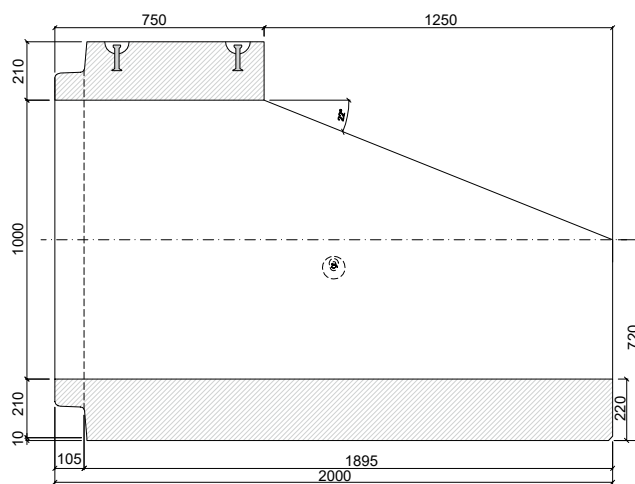
PATKOVÁ TROUBA TZP-SP 100/200/75 SD
