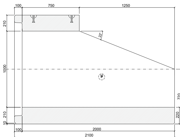
PATKOVÁ TROUBA TZP-SP 100/200/75 SH
