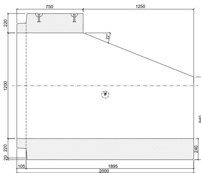
PATKOVÁ TROUBA TZP-SP 120/200/75 SD
