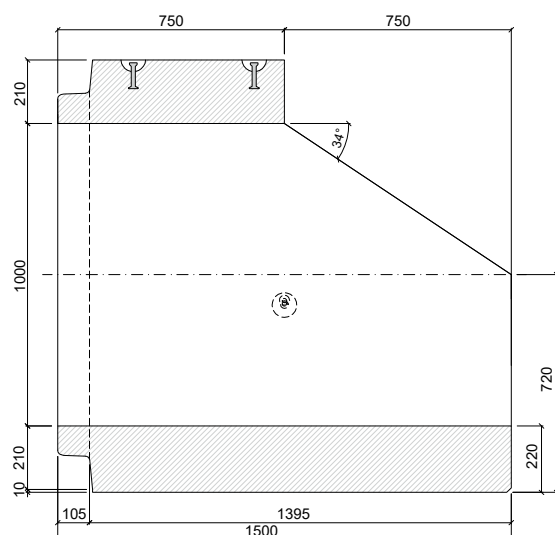
PATKOVÁ TROUBA TZP-ZP 100/150/75 SD
