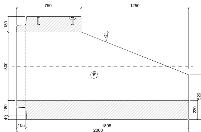
PATKOVÁ TROUBA TZP-SP 80/200/75 SD
