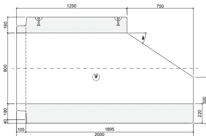
PATKOVÁ TROUBA TZP-SP 80/200/125 SD
