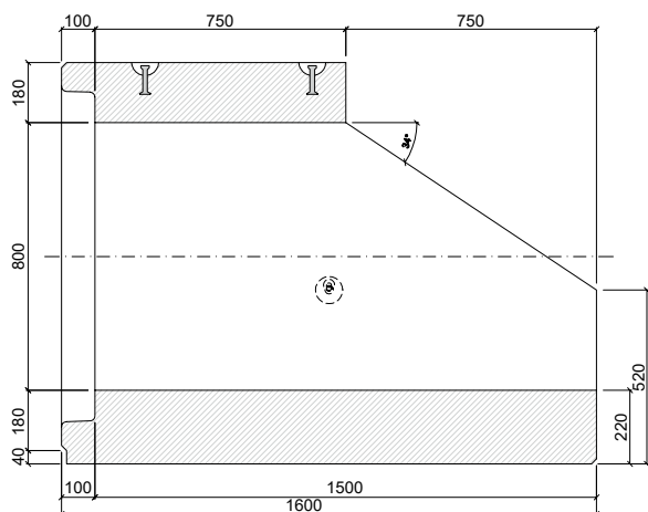
PATKOVÁ TROUBA TZP-ZP 80/150/75 SH
