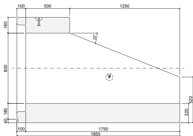
PATKOVÁ TROUBA TZP-SP 80/175/50 SH
