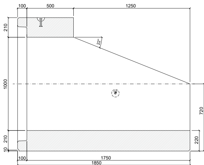
PATKOVÁ TROUBA TZP-SP 100/175/50 SH
