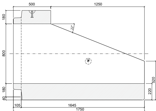
PATKOVÁ TROUBA TZP-SP 80/175/50 SD
