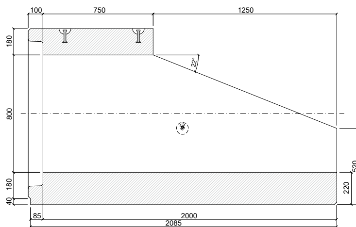
PATKOVÁ TROUBA TZP-SP 80/200/75 SH
