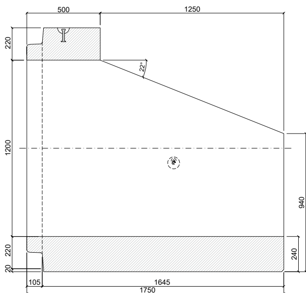
PATKOVÁ TROUBA TZP-SP 120/175/50 SD
