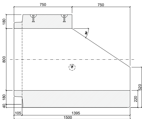
PATKOVÁ TROUBA TZP-SP 80/150/75 SD
