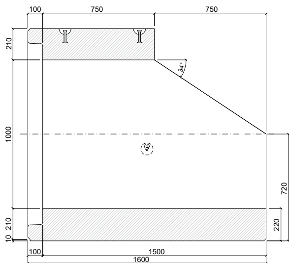
PATKOVÁ TROUBA TZP-ZP 100/150/75 SH
