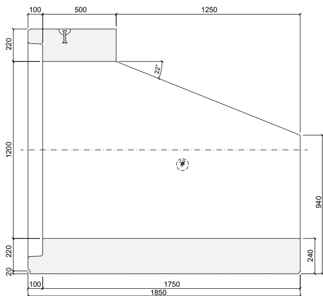
PATKOVÁ TROUBA TZP-SP 120/175/50 SH
