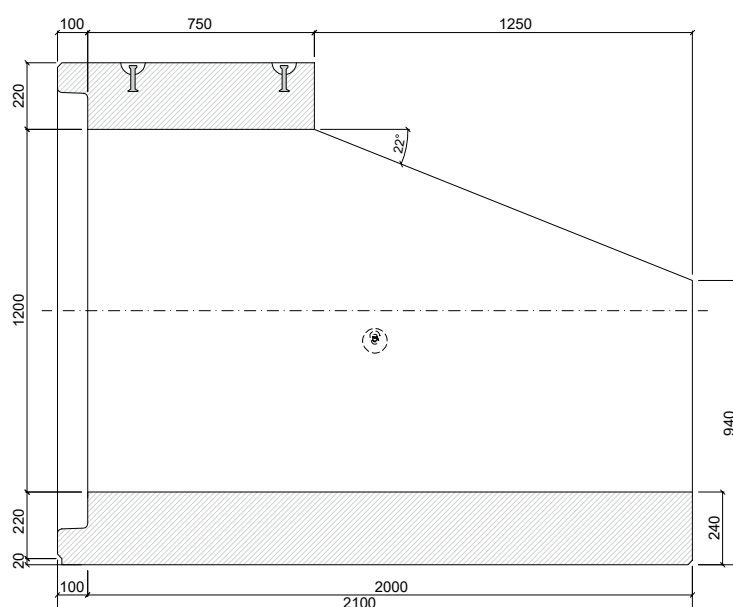
PATKOVÁ TROUBA TZP-SP 120/200/75 SH
